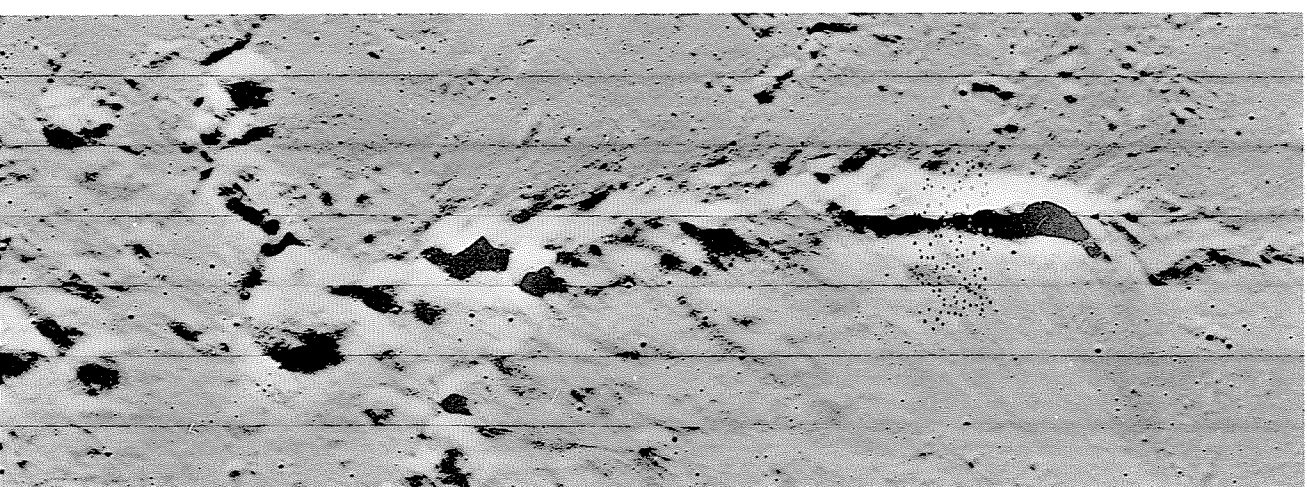
FIGURE 3.4.—Copernicus (93 km, 10° N., 20° W.), the classic locality for study of secondary-impact craters. A. Highly detailed telescopic photograph taken in 1929 by F.G. Pease with the 100-inch telescope of Mount Wilson Observatory. B. Map of secondary craters of Copernicus, constructed in 1960 by Shoemaker (1962b) on basis of photograph in figure 3.4A. C. Lunar Orbiter photograph of Copernicus and northeast exterior, showing rays and subconcentric chains of secondary craters (Rima Stadius I (S), and other secondaries superposed on Mare Imbrium near crater Pytheas (P; 20 km). V-shaped ejecta is downrange from Copernicus at each cluster of secondaries. View southward. Apollo 17 frame M-2444. D. Detail of Rima Stadius I, showing V-shaped herringbone pattern. Orbiter 5 frame M-144.
