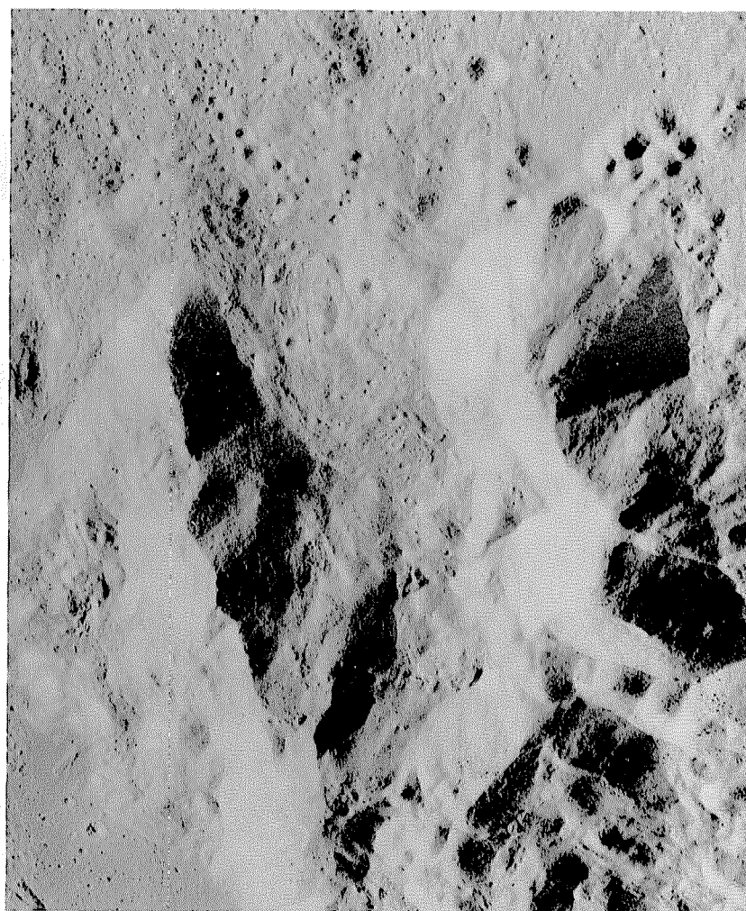
FIGURE 3.32.—Part of "lobster claw" peak of crater King (compare fig. 3.23A), showing superposition of impact melt in gap of peak. Apollo 16 frame P-4998.
