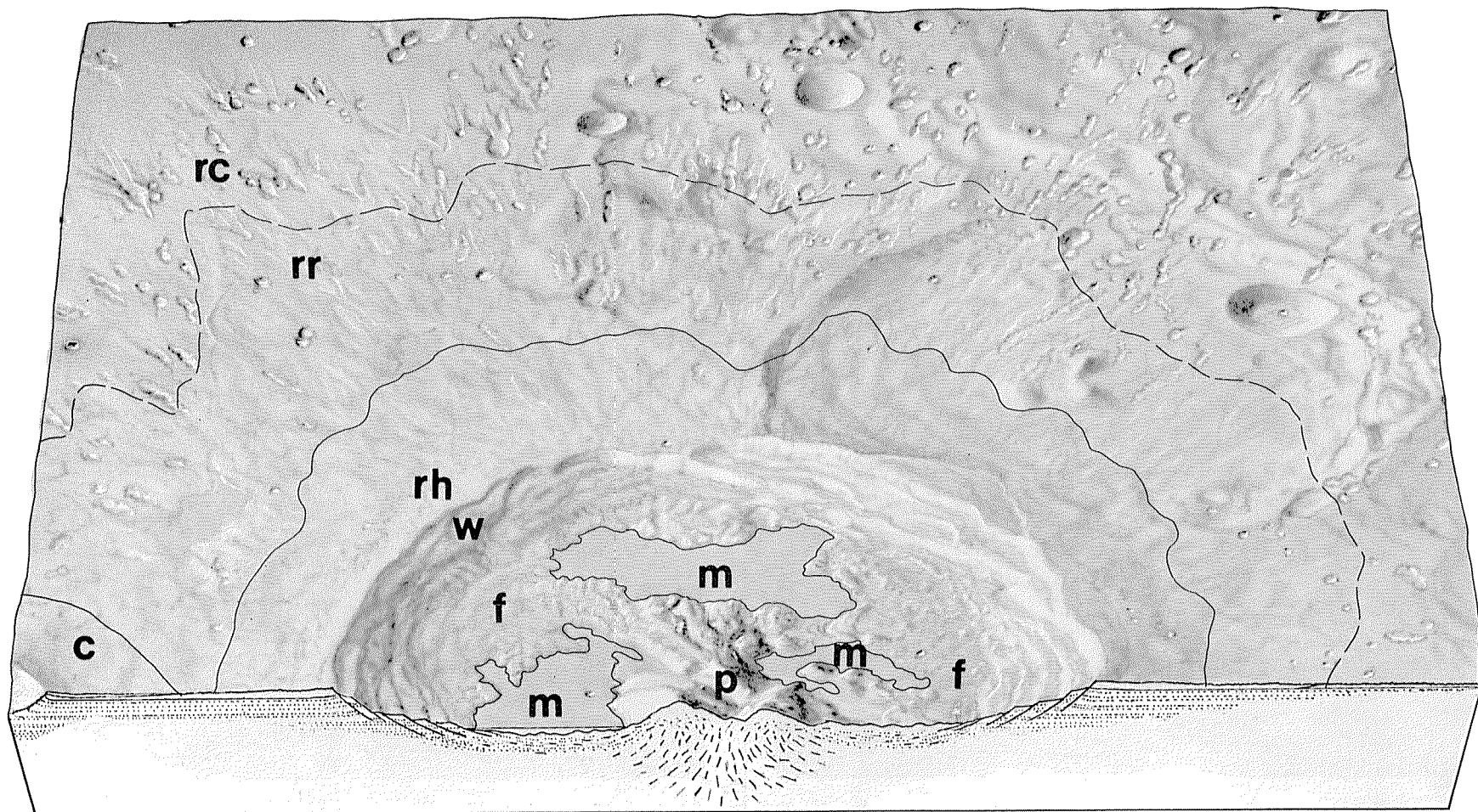
FIGURE 3.22. — Material subunits of a typical large crater, modeled after craters Theophilus and Mädlar. Rim materials are three-dimensional deposits, from rim crest outward: rh, hummocky; rr, radial; rc, cratered (secondary craters). Structural units, not sharply demarcated in subsurface, are floor material (f), peak material (p), and wall material (w). Planar impact-melt rock (m) overlies other units. Material of simple crater (c) overlies unit rr. Drawing by Donald E. Davis, courtesy of the artist.
