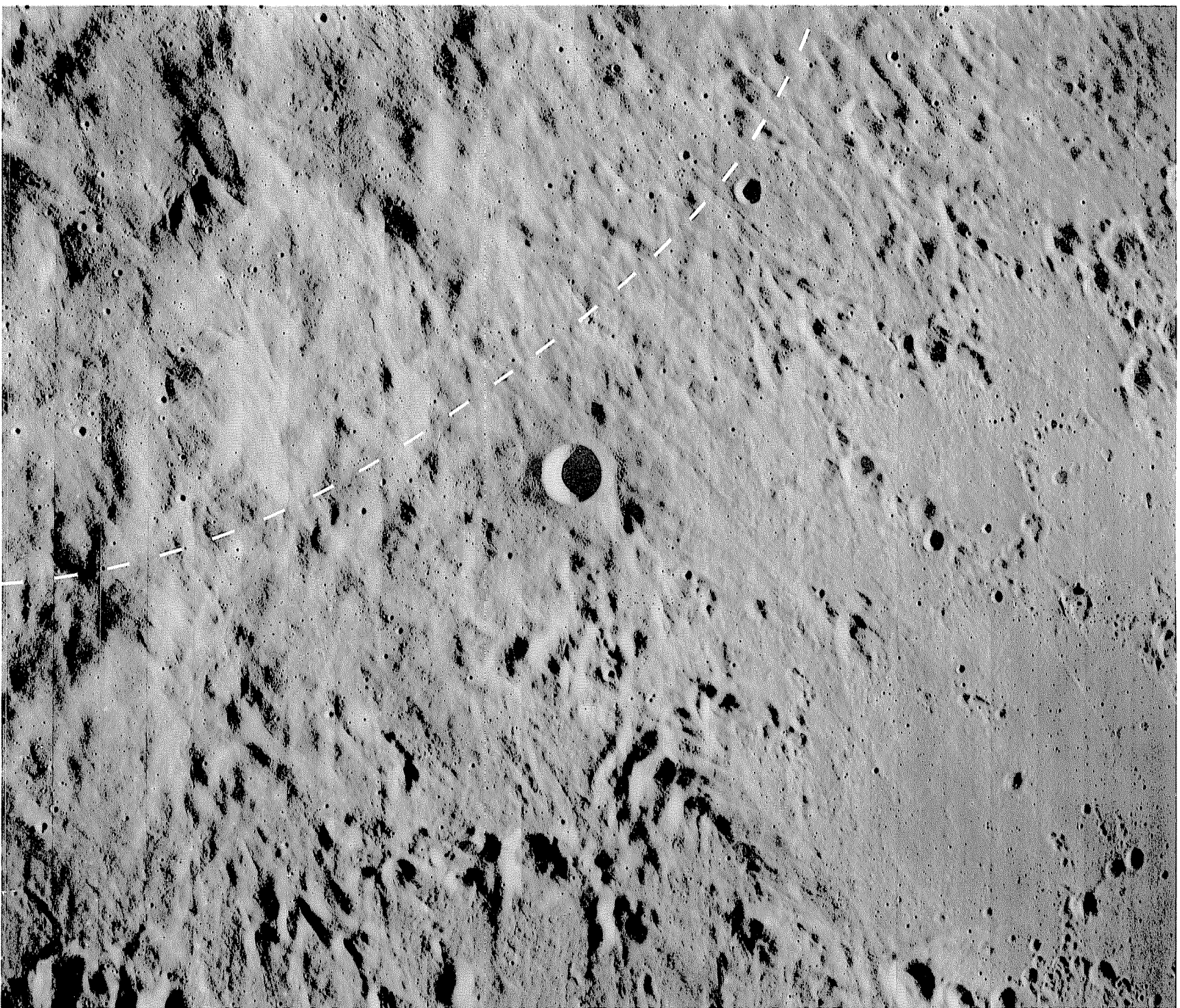
F. Southeast sector of Copernicus. Conspicuous secondaries with herringbone pattern lie mostly beyond (to right of) one crater radius (white dots). Superposed crater in center is Copernicus H (4.3 km; see chap. 13). Orbiter 5 frame M-147.
