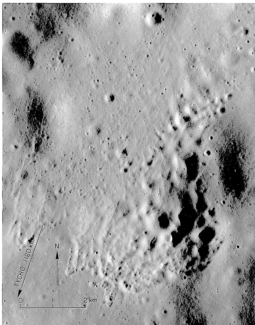
FIGURE 3.6.—Cluster of crisp-textured secondary craters of Tycho (on east rim of Ptolemaeus at 9.2^\circ S., 1.0^\circ E.). Fine herringbone pattern is evident above directional arrows. From Lucchitta (1977a). Apollo 16 frame P-4653.
