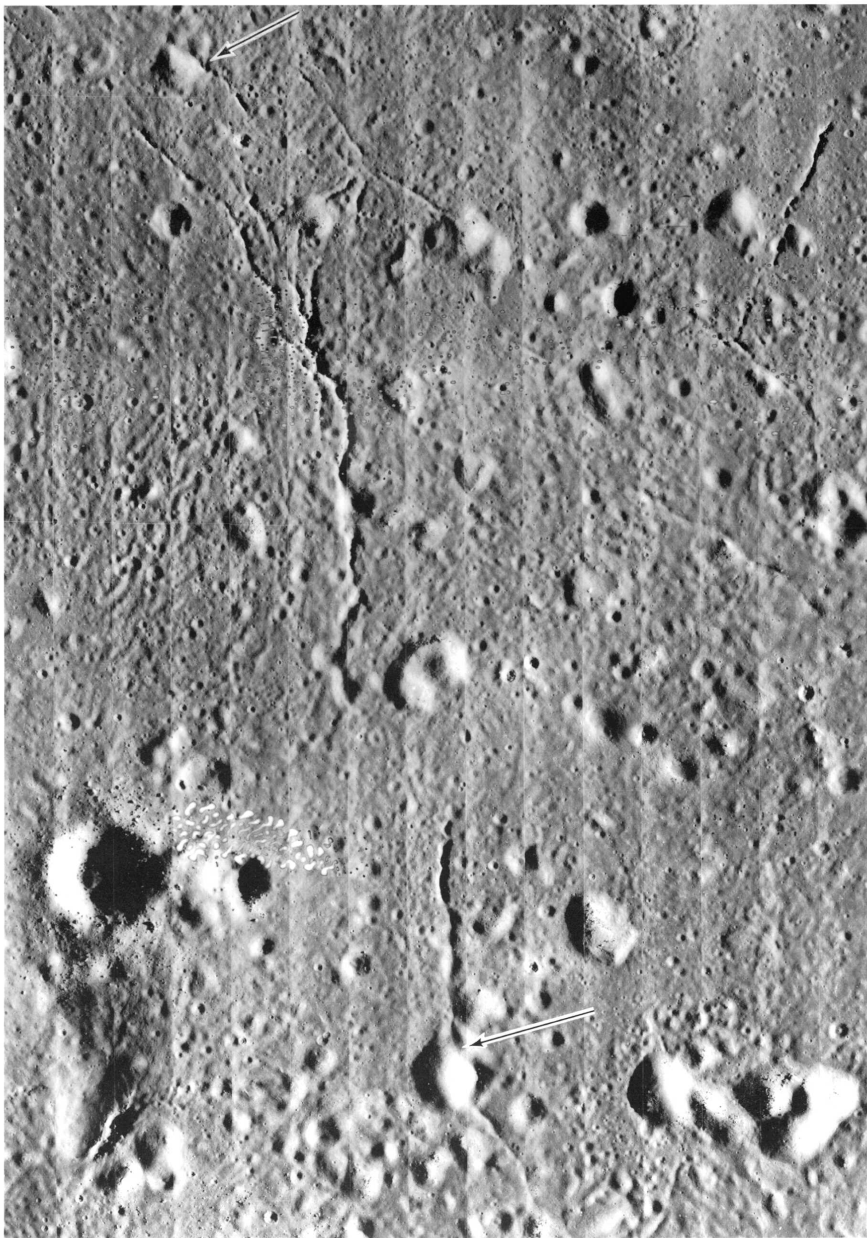
FIGURE 3.35. — Impact melt and floor mounds of Copernicus; melt is superposed on mounds at arrows. Fissures indicate shrinkage of melt and, possibly, drainage into subsurface cavities. Orbiter 5 frame H-153.
