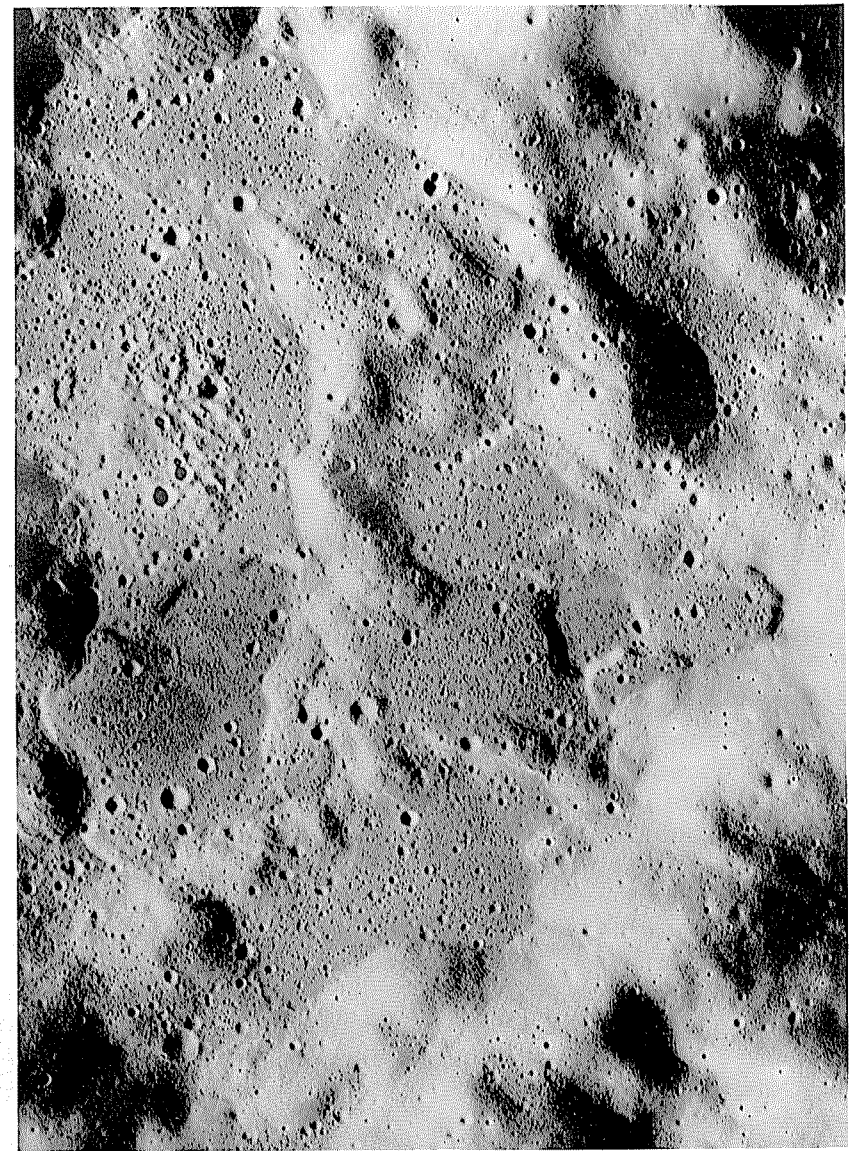
FIGURE 3.27.—Eastern ejecta of Tsiolkovskiy (180 km).
