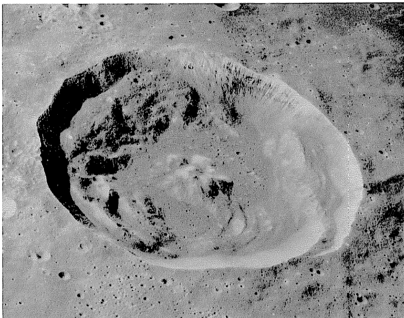
FIGURE 3.29.—Crater Euler (28 km, 23° N., 29° W.), showing wall materials weakly coalesced into terraces at bottom and uncoalesced in upper left. Precrater stratigraphic units are evident by albedo differences on upper right wall. Apollo 15 frame P-10274.
