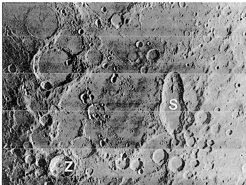
FIGURE 3.11.—Irregular primary-impact craters.
