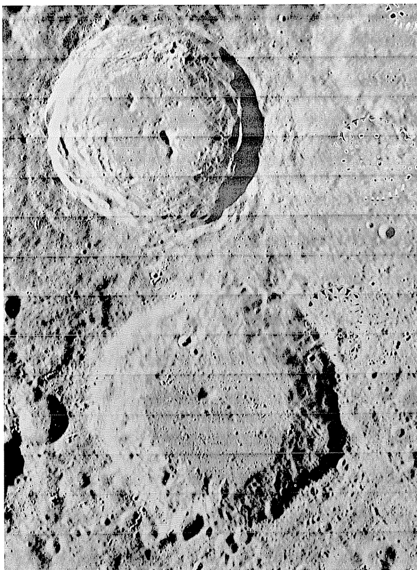
FIGURE 3.26.—Ejecta of moderately fresh (Eratosthenian) crater Werner (70 km, 28° S., 3° E., above), superposed on crater Aliacensis (80 km, below), whose subdued walls, raised rim wreath, and central peak were probably similar to those of Werner when first formed; Aliacensis-radial ejecta is no longer visible. Rim nearest Werner is more highly degraded than distal rim. Orbiter 4 frame H-100.
