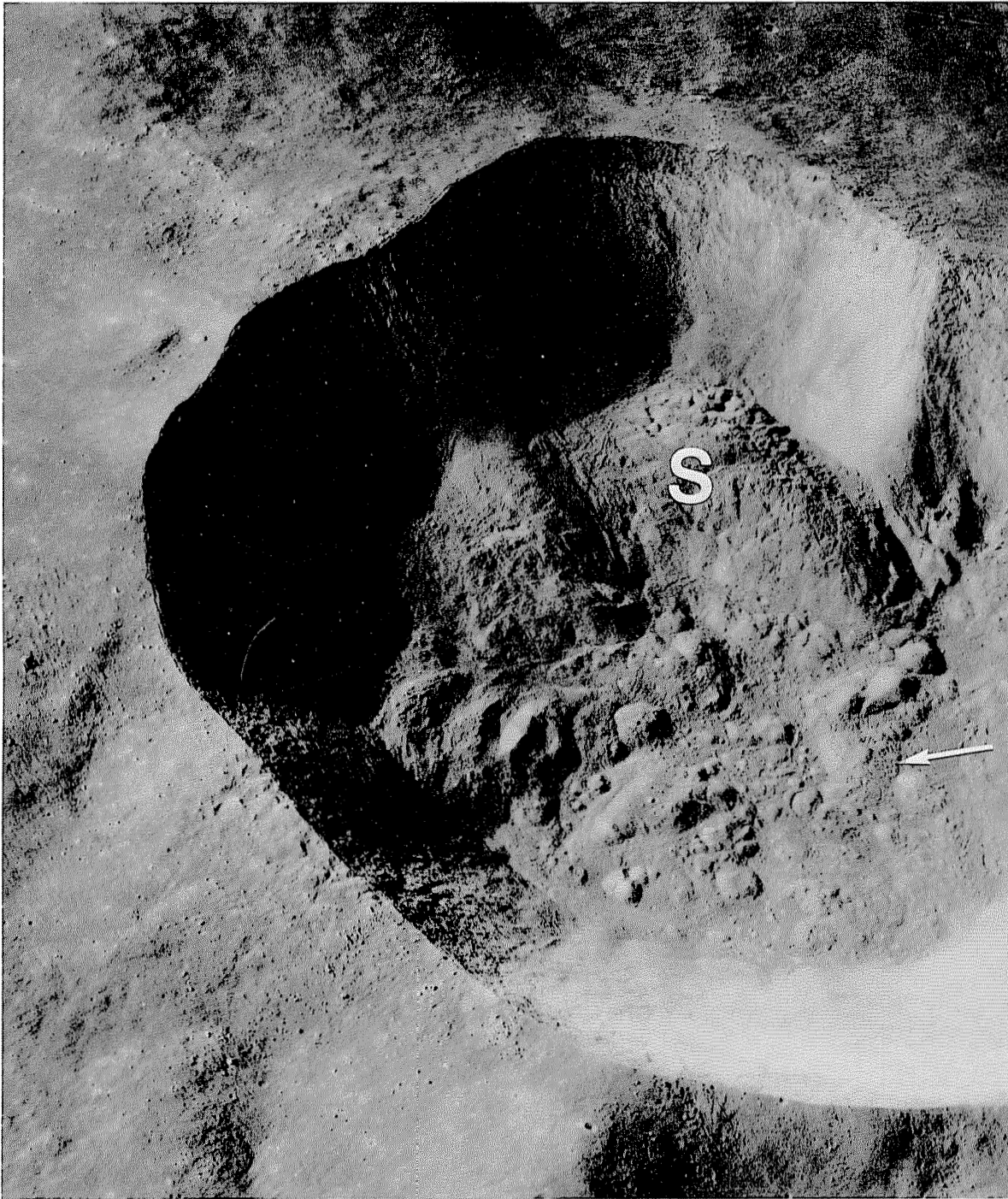
FIGURE 3.33.—Crater Proclus (28 km, 16° N., 47° E.), showing terrace-free walls, slump from upper wall (S), coarse floor mounds probably produced by floor uplift, and fissured impact melt on floor (arrow). Apollo 17 frame P-2265.
