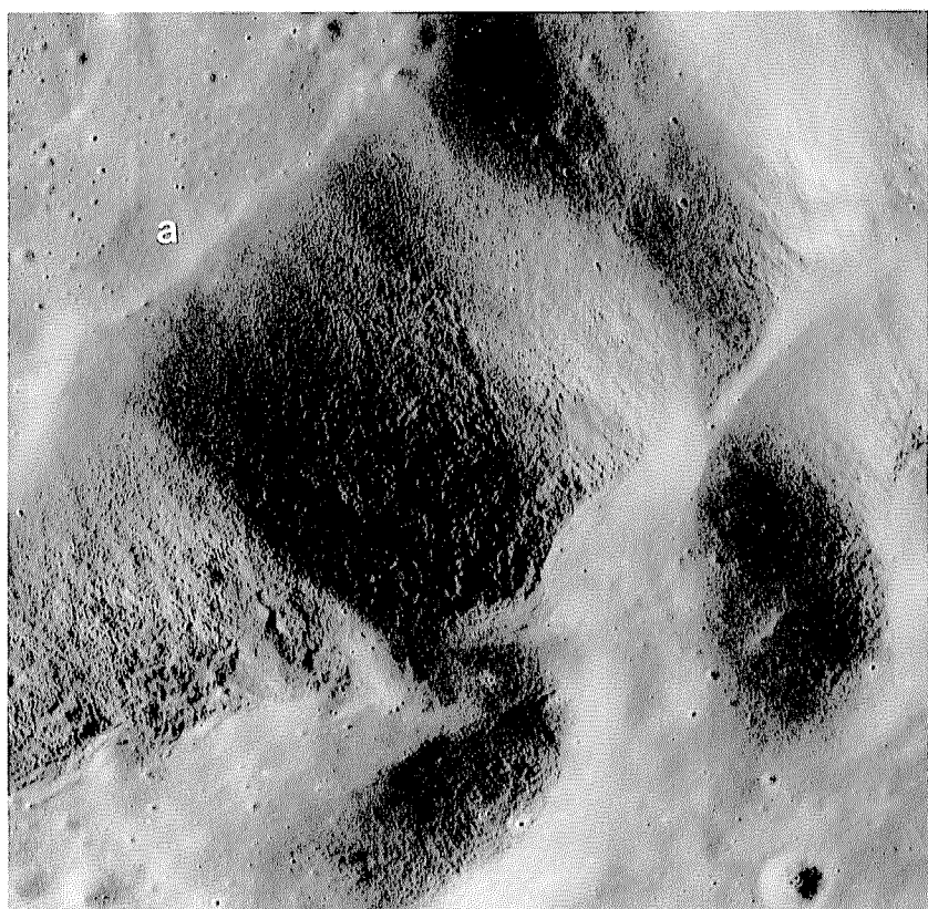
FIGURE 10.11.—Part of Montes Apenninus, showing paucity of outcrops and blocks on slope, and colluvial apron at base (a). Apollo 15 frame P-9804.
