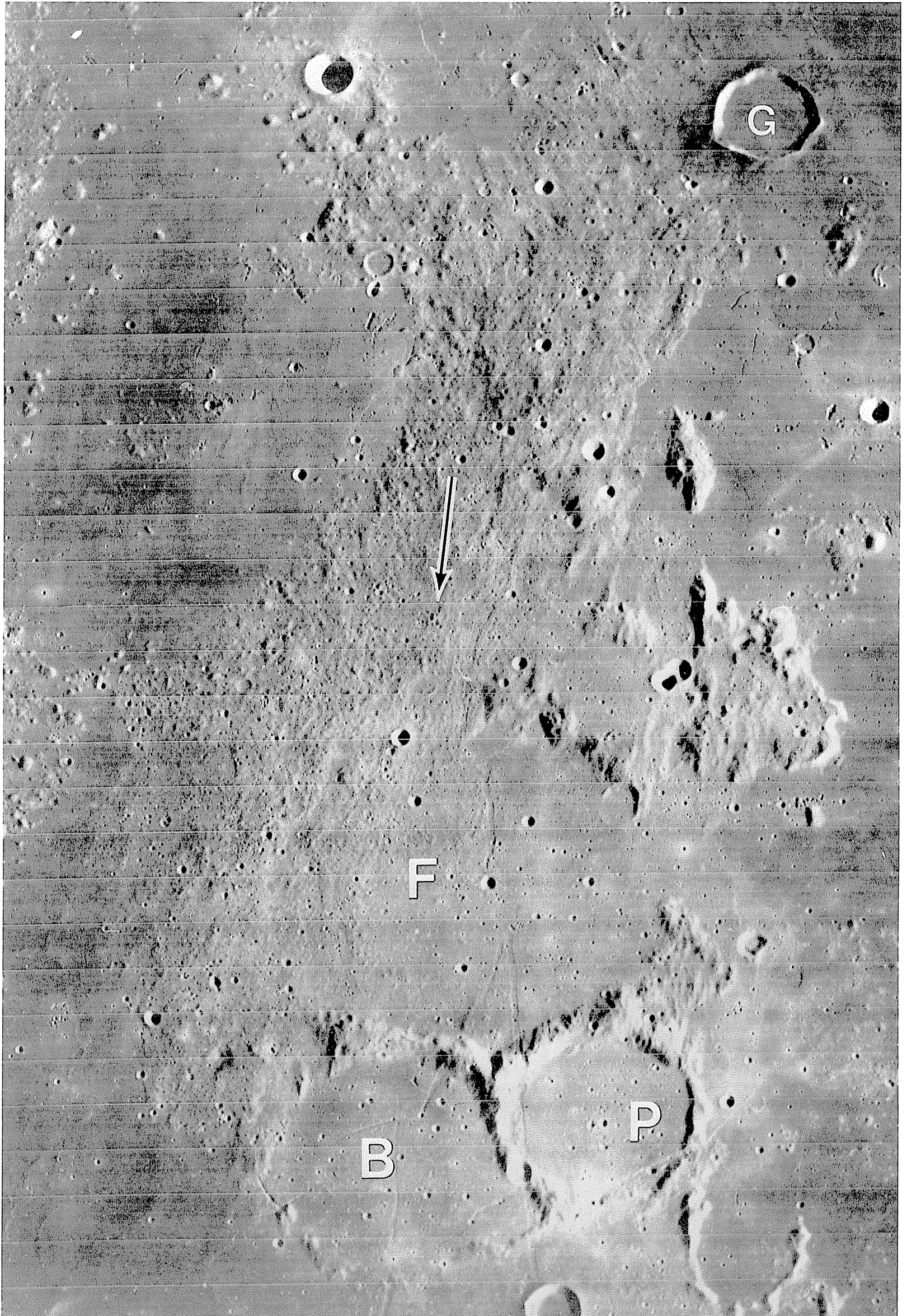
FIGURE 10.19. — Type area of the Fra Mauro Formation. Arrow, Apollo 14 landing site. Fra Mauro Formation, Imbrium sculpture, and plains deposits overlie pre-Nectarian or Nectarian craters Fra Mauro (F; 95 km), Bonpland (B; 60 km), and Parry (P; 48 km); Fra Mauro Formation is overlain by Imbrian crater Gambart (G; 25 km, 1° N., 15° W.). Orbiter 4 frame H-113.
