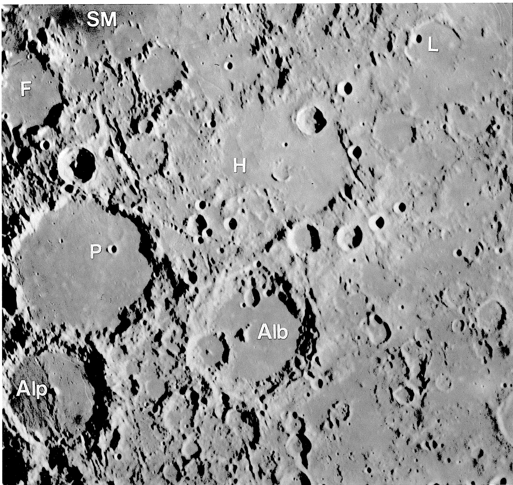
FIGURE 10.27. — Imbrium sculpture in south-central nearside highlands south of Sinus Medii (SM). Craters cut by sculpture include Lade (L; compare figs. 10.16, 10.17), Flammarion (F; 75 km), Hipparchus (H; 151 km), Ptolemaeus (P; 153 km), Albategnius (Alb; 136 km, compare figs. 10.29, 10.36), and Alphonsus (Alp; 119 km). Planar fill apparently transects sculpture. Subcircular secondary craters of Imbrium are visible below latitude of Ptolemaeus. Catalina Observatory photograph No. 1907.
