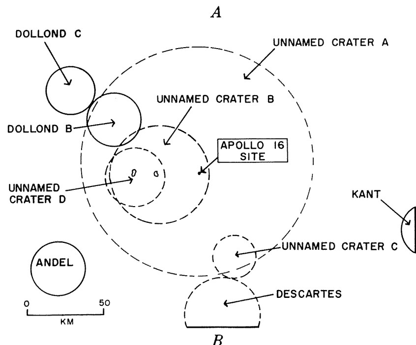
FIGURE 10.40.—Vicinity of Apollo 16 landing site.
