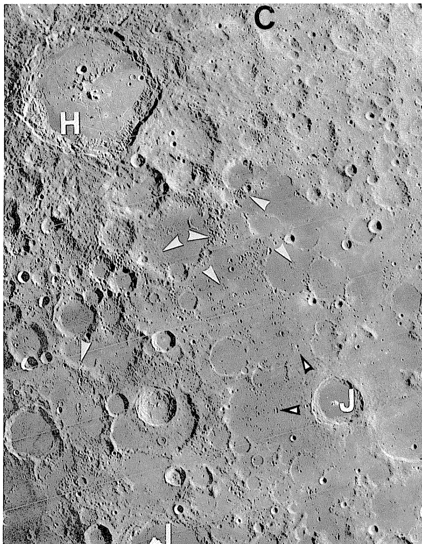
FIGURE 10.46.—Stratigraphic relations of mare and crater materials in Mare Australe. A. Deposits of Jenner (J; 72 km, 42° S., 96° W.) and Humboldt (H; 207 km, 27° S., 81° E.), both Upper Imbrian, are superposed on mare basalt (white-on-black arrowheads), whereas a younger mare unit encroaches on Humboldt secondaries (white arrowheads). C, pre-Nectarian crater Curie (139 km, 23° S., 92° E.); L, pre-Nectarian crater Lyot. Orbiter 4 frame M-9.
