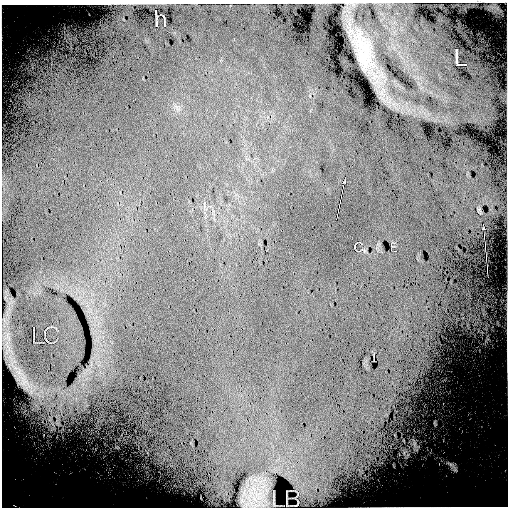
FIGURE 10.41.—Imbrian craters on periphery of Imbrium basin. Lansberg (L; 39 km, 0.3° S., 26.5° W.) is superposed on hummocky Imbrium ejecta (h) and embayed by mare materials (arrows). Interior and periphery of Lansberg C (LC; 17 km) are flooded more deeply. Rayed, probably Copernican, but somewhat degraded crater Lansberg B (LB; 9 km) is superposed on the mare. Craters in 1-km size range are probably Imbrian (I), Eratosthenian (E), and Copernican (C). Apollo 12 frame H-8095.
