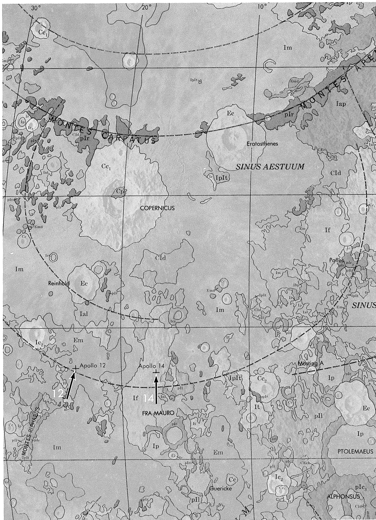
FIGURE 10.18.—Part of geologic map of lunar nearside (Wilhelms and McCauley, 1971), including Apollo 12 and 14 landing sites (arrows). If, Fra Mauro Formation; Em, Eratosthenian mare material (Apollo 12; see chap. 12). Montes Carpathus, 550 km north of Apollo 14 landing site, constitutes south rim of Imbrium basin. Ring passing near landing sites is part of Insularum basin in one interpretation, but may be ring of Procellarum basin (see chap. 8; pls. 3–7).
