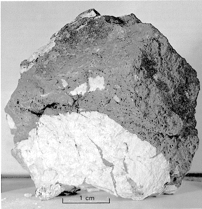
FIGURE 10.13. —“Black-and-white” breccia sample 15455 from rim of Spur Crater, station 7, Apollo 15 landing site. Black component is impact melt, probably formed by Imbrium impact (Ryder and Bower, 1977). White component is pre-Nectarian anorthositic norite (table 8.4).
