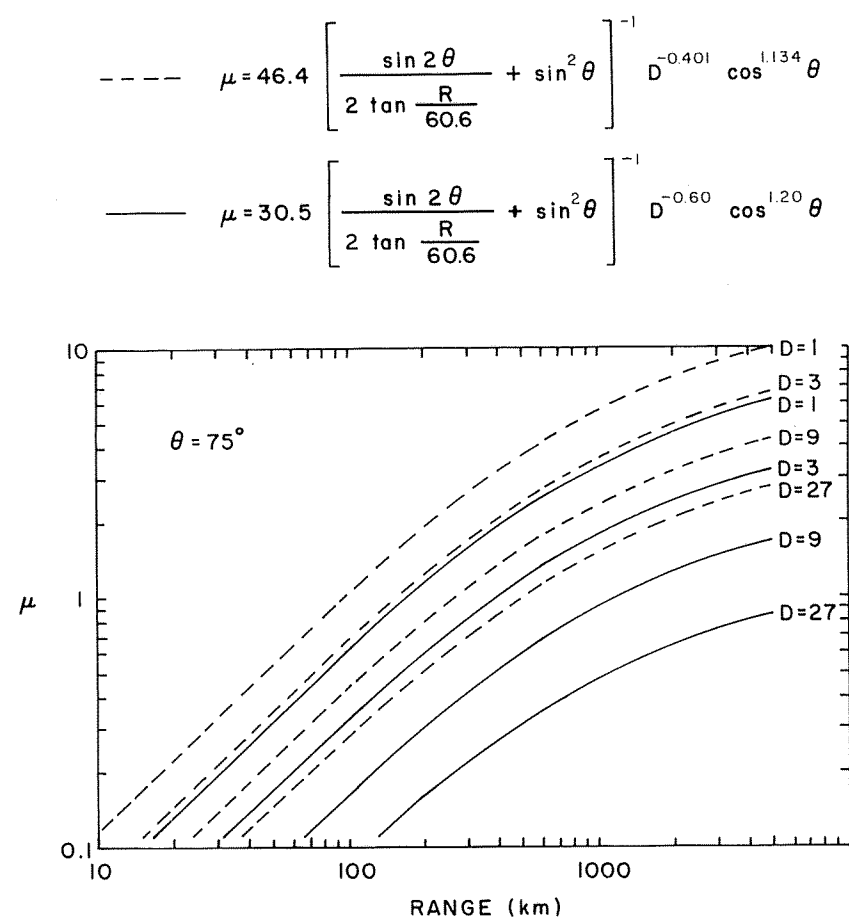
FIGURE 10.26.—Mass ratio of primary versus local material as a function of range from source of incoming ejecta. Dashed lines are based on upper equation, which assumes scaling of D = KE^{-3.4} (Oberbeck and others, 1975); solid lines are based on lower equation, which assumes scaling of D = KE^{-3.6} (H.J. Moore, written commun., 1980). \mu , ratio of mass ejected from secondary crater to mass of ejecta projectile that created crater; \theta , angle of impact (equal to angle of ejection), measured from local surface normal; D , diameter of secondary crater (in kilometers); R , range or distance along Moon's surface from point of ejection within primary crater or basin to secondary crater (in kilometers). Courtesy of H.J. Moore.
