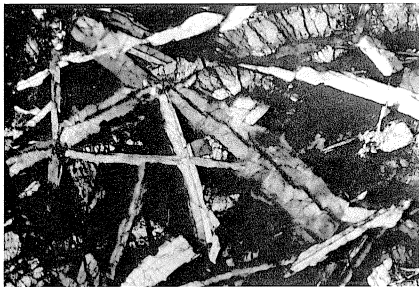
FIGURE 10.10.—Thin section of crystalline, probably volcanic KREEP-rich sample 15386,8, showing basaltic intersertal to subophitic texture (Dowty and others, 1976). Fragment lacks clastic inclusions and meteoritic siderophile elements (Irving, 1975, 1977; Dowty and others, 1976). Crossed polarizers; field of view, about 2 mm.
