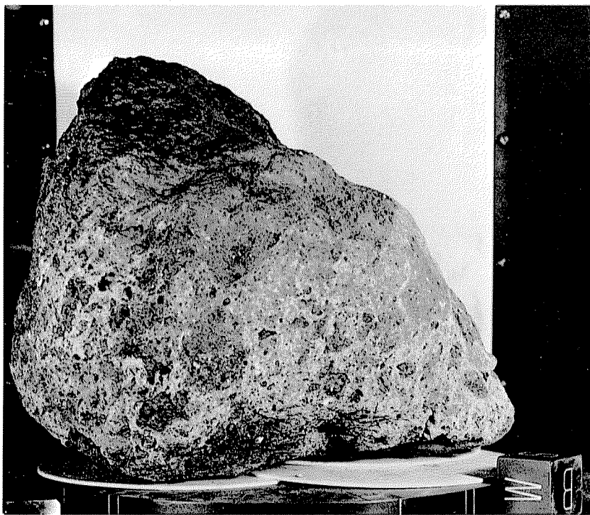
FIGURE 10.24.—Large (8.9 kg) Fra Mauro breccia sample 14321, "Big Bertha," from rim of Cone Crater, Apollo 14 landing site: a polymict breccia displaying multiple episodes of brecciation (Duncan and others, 1975; Grieve and others, 1975). A. Entire hand specimen, showing complex relations of clasts and matrix.
