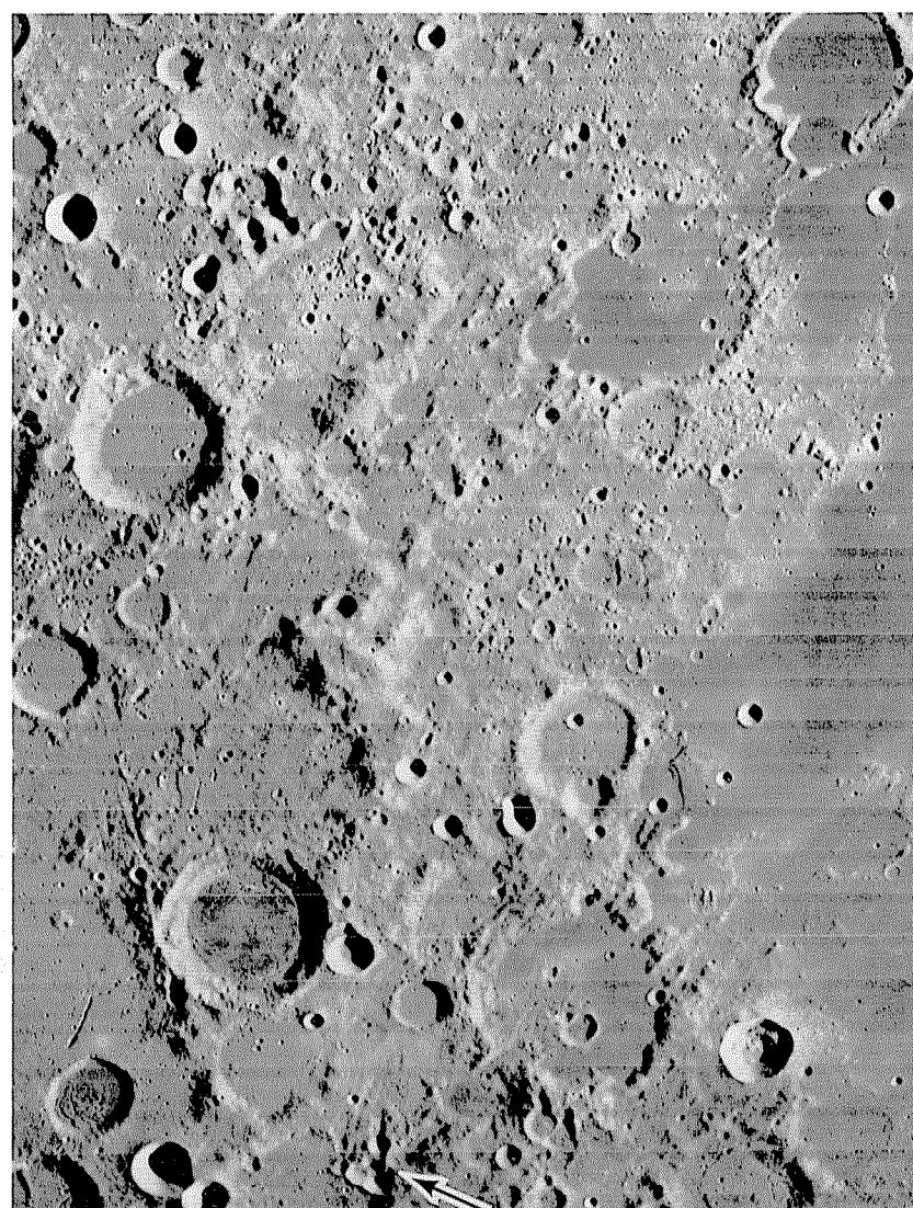
B. Detailed view of Orientale-secondary craters, showing herringbone-patterned ejecta interrupting Imbrium-radial chains (arrow at bottom). Orbiter 4 frame H-189.
