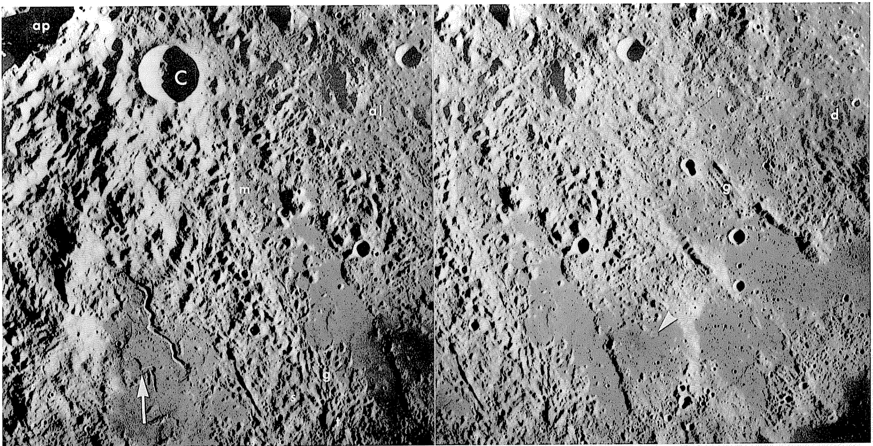
FIGURE 10.14. —Types of Imbrium ejecta on flank of Montes Apenninus. ap, northwest-facing Apennine scarp. Concentric “material of Montes Apenninus” is closest to scarp; farther out are knobby Alpes Formation (al), radially grooved terrain (g), smooth terrain (s), transverse fissures (f), and level ponds of probable impact melt (m). Arrows, irregular craters in mare, including “D caldera” (arrowhead in right frame; chap. 5; compare fig. 5.10 D ); d, dark-mantling material. C, fresh crater Conon (22 km; compare fig. 10.7). Stereoscopic pair of Apollo 17 frames M-1821 (right) and M-1823 (left). From Wilhelms (1980, fig. 13).
