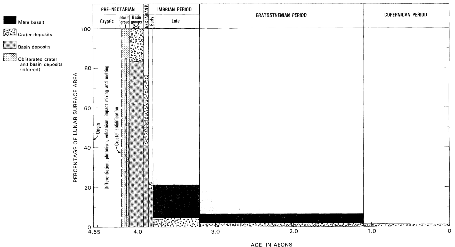
FIGURE 14.3. — Evolution of the lunar surface. Vertical axis, surface area inferred to have been originally covered by each group of deposits. Basin and crater deposits (approximately, the continuous ejecta) are assumed to extend one diameter from the crater or basin center; mare deposits of each age are assumed to extend beneath entire area of younger maria. Procellarum and South Pole-Aitken basins (pre-Nectarian basin group 1) are shown diagrammatically by narrow vertical bars; ages are estimated. Observed and inferred pre-Nectarian crater deposits cover more than 100 percent of the Moon. Early peak in lunar geologic activity is evident.
