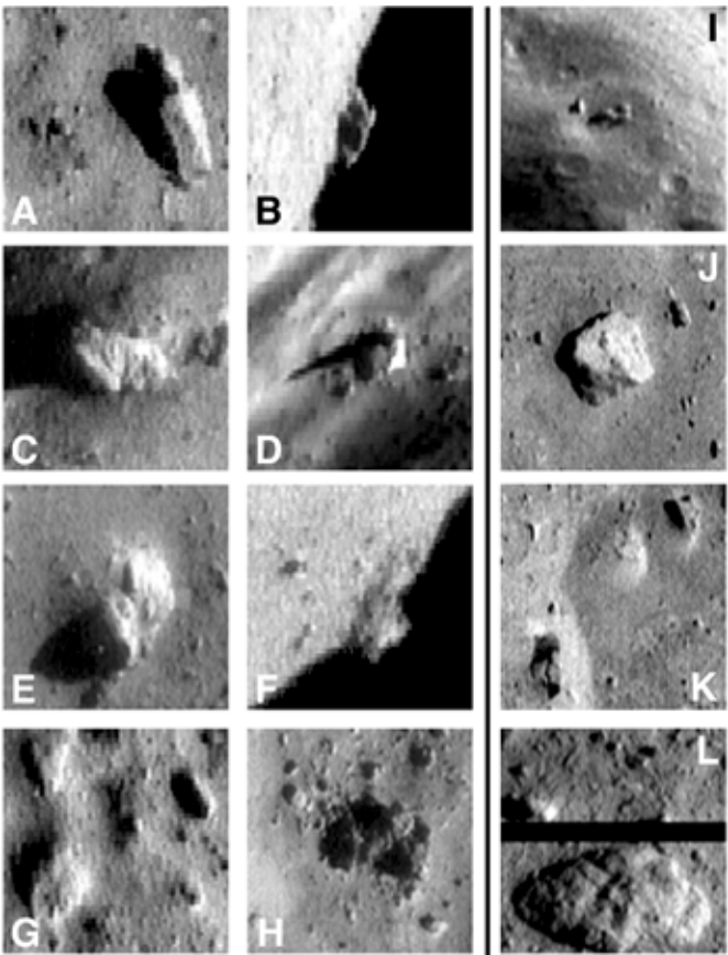
FIG. 16. ( left ) Boulders on Eros exhibit a wide spectrum of physical properties (a–h) from sharp angular coherent boulders to disintegrating loosely bound rubble piles (Table 4). We interpret this range of coherence to reflect variations of coherence with depth in the Eros regolith. (i) Grouping of 60–80 m diameter boulders (inside 1000 m diameter degraded crater); see oblique view in upper left of Fig. 12. (j) Angular 36 m boulder. Square shapes of boulders may indicate an organized joint pattern inside Eros consistent with a relatively intact interior. (k) Fractured boulder at lower left is ~20 m long; this example is reminiscent of boulders investigated on the Moon by Apollo astronauts. The fracturing of the lunar boulders was thought to have occurred as the boulder impacted at relatively low velocities as a secondary—the same is most certainly true for the Eros example shown here (and many others). (l) Rounded, partially buried 16 m (left to right) boulder showing fractures (or joints) spaced ~1 m. The black stripe across framelet represents data lost in transmission (–40.7° S, 275.7° W; Table 3 for relevant image parameters).
