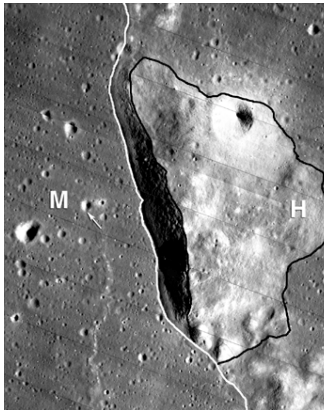
FIG. 5. Lunar Orbiter frame (LO3 200M) used in crater counting. Mare area delineated with white line and labeled "M", highland area marked with "H" and black outline (small crater marked with arrow centered at 2.8° S, 317.5° E, frame width ~10.6 km, 6.7 m/pixel, incidence angle ~71°).
