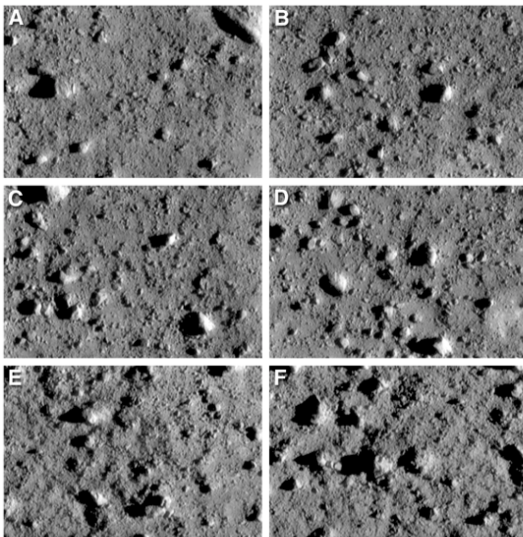
FIG. 24. During NEAR Shoemaker's descent to the surface extremely high-resolution imaging was obtained that reveals the regolith in great detail. Contrast the surface seen here with that in Shoemaker Regio shown in Fig. 11c at 10× coarser resolution (~3 m/pixel). (a) 157416918; width of frame ~36 m; (b) 157416938, width of frame ~35 m; (c) 157416983, width of frame ~33 m; (d) 157417003, width of frame ~31 m; (e) 157417048, width of frame ~27 m; (f) 157417068, width of frame ~25 m.
