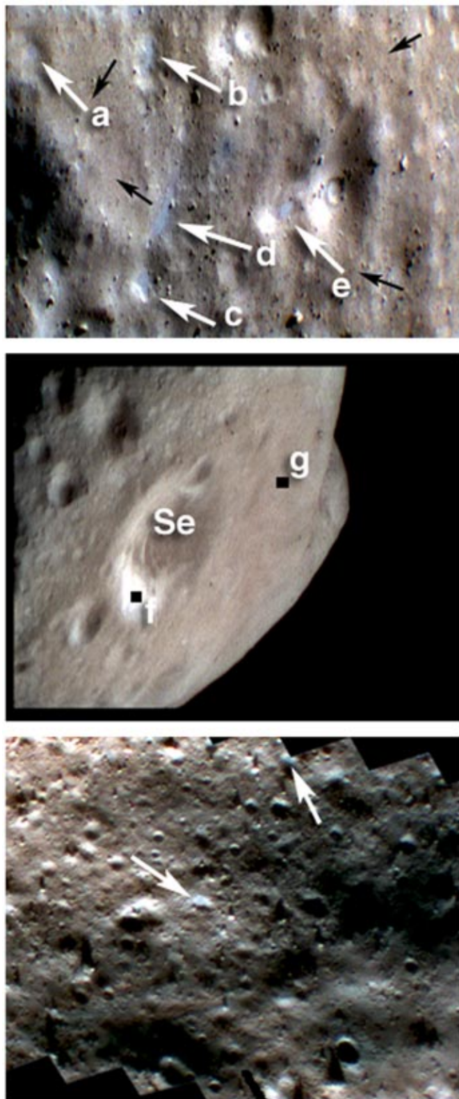
FIG. 21. (Left) (top) Ponded sedimentary deposits ("ponds") on Eros exhibit distinct color properties relative to their surroundings; in this saturation stretch color ponds show up as smooth blue deposits occupying topographic lows. At the center of the frame incidence angle is 47^\circ and the phase angle is 86^\circ . Located at latitude 9.8^\circ S, longitude 32.4^\circ W. Spectral samples of each pond (white arrows indicate sampled ponds "a" 3 \times 3 pixel sample, "b–e" 5 \times 5 pixel samples) and surrounding intercrater terrain (black arrows, 9 \times 9 sample boxes—see also Figs. 22, 23 and Table 5; METs = 154760995F1, 154760999F3, 154761001F4, width of frame 1.13 km). (middle) Ponds share color properties with high-albedo patches found on many steep crater walls. In this oblique view of Selene crater (3.1 km diameter) spectral sample areas are marked with black boxes, "f" is 9 \times 9 pixel average while "g" is a 51 \times 51 pixel average (see Fig. 23; Table 5; METs = 151926384F1, 151926386F3, 151926388F4). Here the ponds show a \sim 6\% reflectance contrast (top panel) with their surroundings while the bright material in Selene exhibits a 60\% increase in reflectance relative to the surrounding terrain. (bottom) Shoemaker Regio was probably formed as a result of fallback material during the formation of Shoemaker crater with subsequent remobilization by downslope movement events (see Fig. 11a–c). Despite the abundance of regolith materials, ponds do not form efficiently in this environment, perhaps due to the predominance of steep slopes and relatively frequent reworking of materials? However, small ponds (arrows) can be found in high-resolution images and they share the same color properties (Fig. 23) as ponds found elsewhere on Eros (METs = 155091985F1, 155091987F3, 155091989; distance from arrow-tip to arrow-tip 770 m, lower pond located at 19.32^\circ S, 309.60^\circ ). In all three panels colors formed as red 950 nm, green 760 nm, and blue 550 nm.
